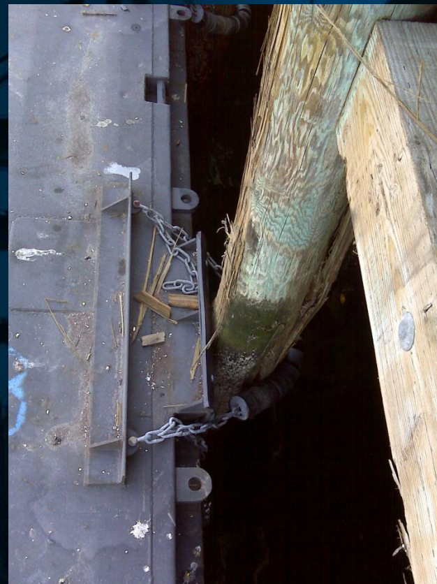
Deterioration of Existing Timber system (East Berth)
